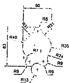
CUTOUT DETAIL SCALE: 1:10
