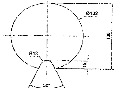
CUTOUT DETAIL SCALE: 1:10
