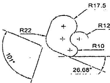
CUTOUT DETAIL SCALE: 1:10
